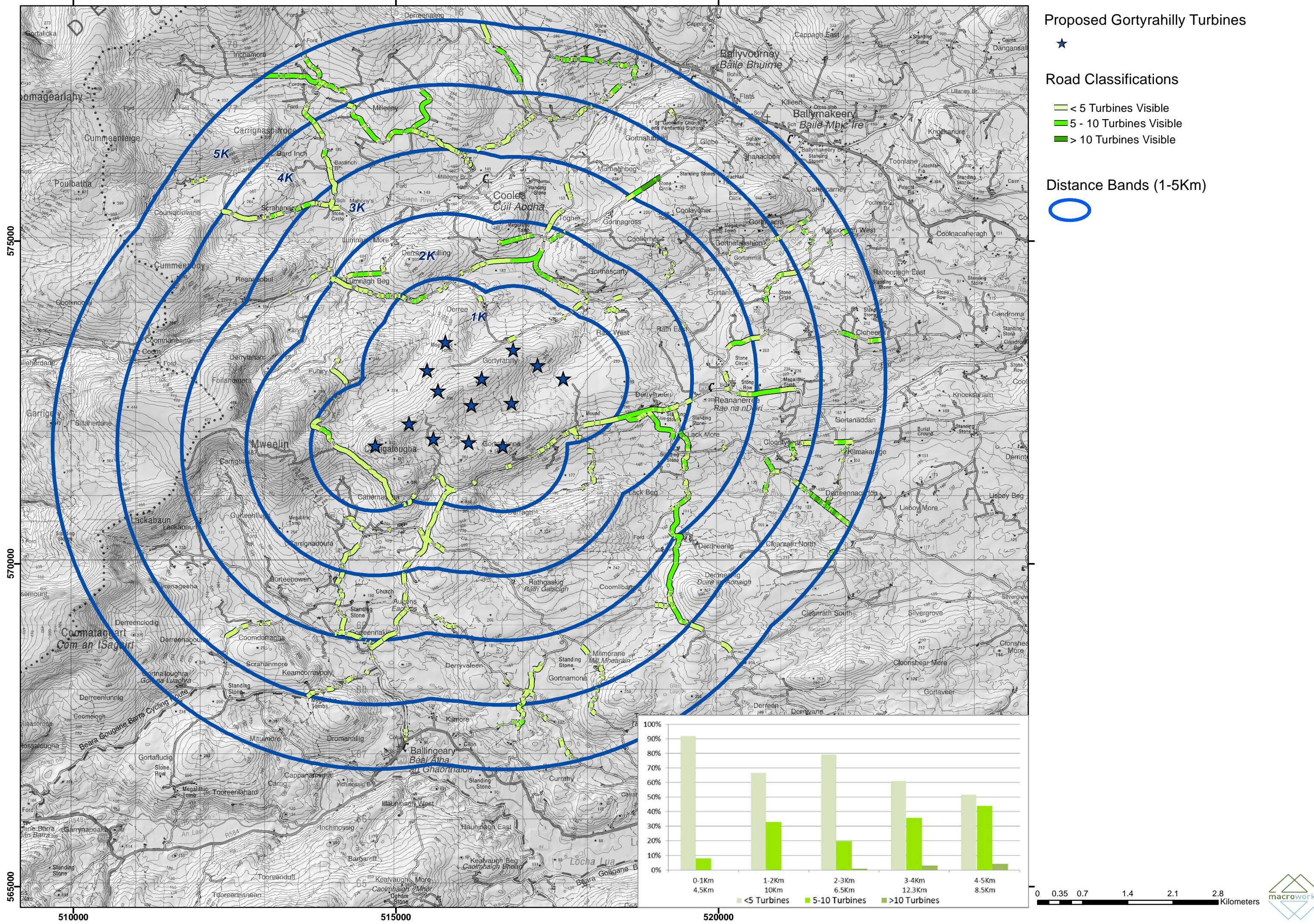
Figure 12.5 RSA "Open View" Refinement Map
